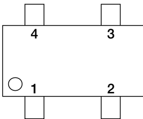
SC-82ABB (TOP VIEW)
