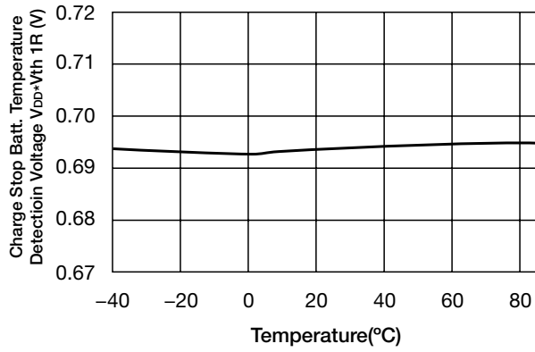
■ Charge Recovery Batt. Temperature Detection Voltage
