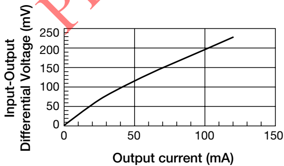
■ Input-Output Differential Voltage
