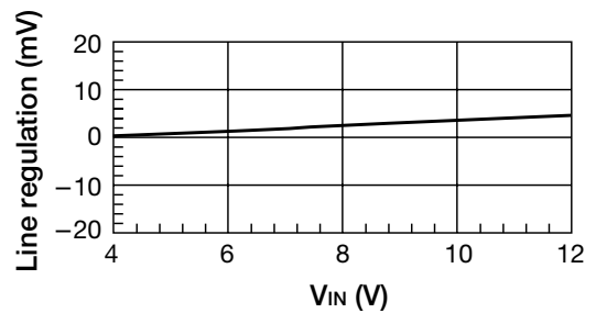
■ Line Regulation
