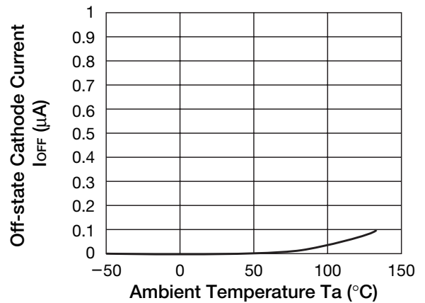
Off-stage Cathode Current vs T_a
