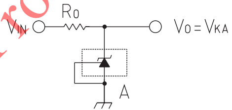
(3) Off-stage Cathode Current Test Circuit
