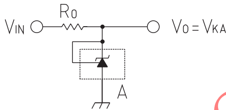
(1) Reference Voltage Test Circuit
