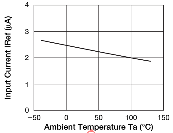
Input Current vs T_a
