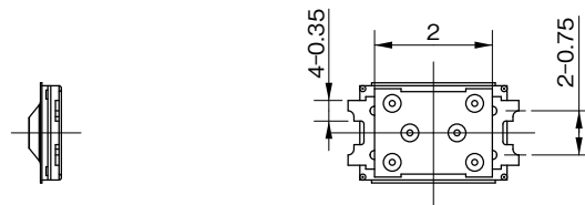
Reference solder mask stencil dimension
