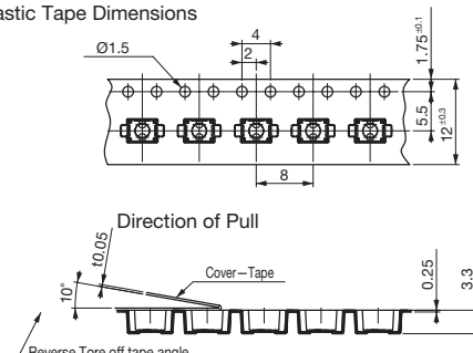
Fig-3 TOLERANCE ±0.1
