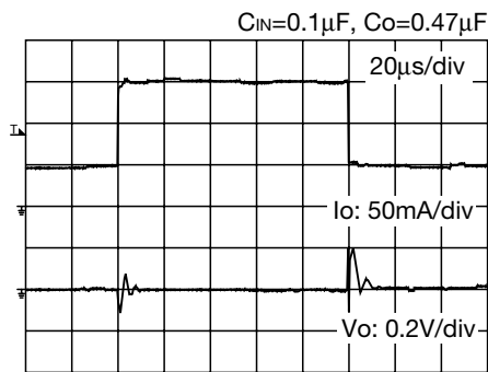
■ Load transient response V_{O1} ( I_o=50 \rightarrow 150\text{mA} )
