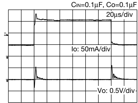
■ Load transient response V_{O2} ( I_o=50 \rightarrow 150\text{mA} )
