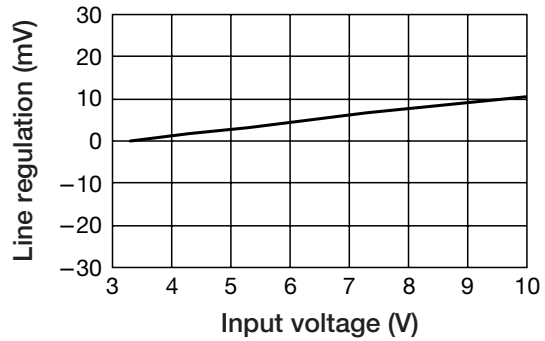
Line Regulation
