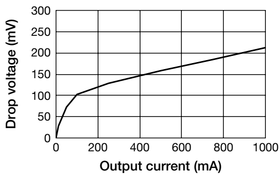
Drop Voltage
