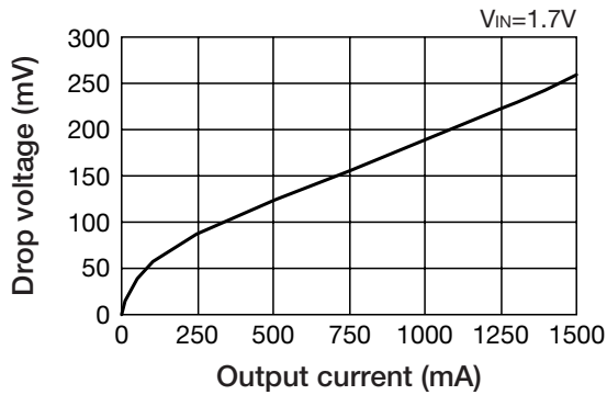
Drop Voltage
