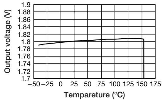
Temperature-Output Voltage
