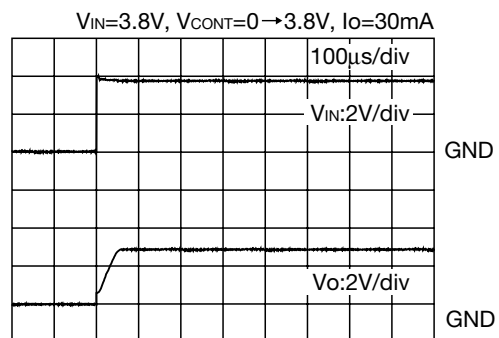
■ Turn-On Transient Responses
