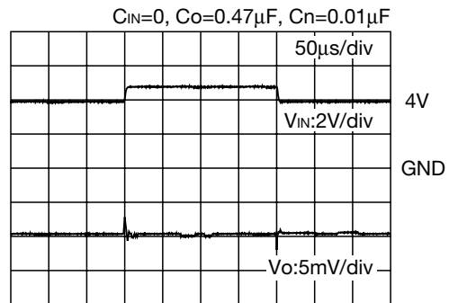
■ Line Transient Responses ( V_{IN}=3.8 \rightarrow 4.8V , I_o=30mA )
