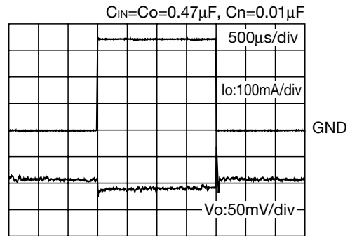
■ Load Transient Responses ( I_o=0 \rightarrow 300mA )
