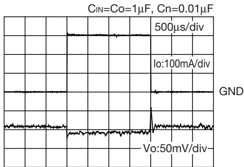
■ Load Transient Responses ( I_o=0 \rightarrow 300mA )
