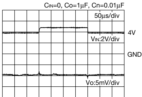
■ Line Transient Responses ( V_{IN}=3.8 \rightarrow 4.8V , I_o=30mA )
