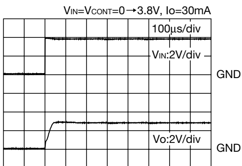
■ Turn-On Transient Responses
