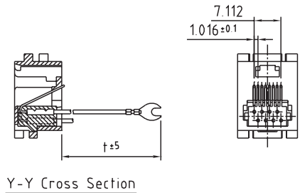
Y-Y Cross Section
