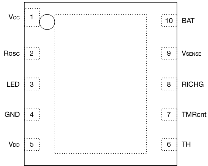
PLP-10A (TOP VIEW)
