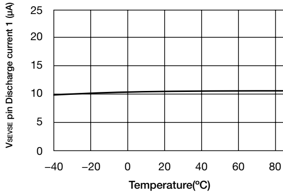
V SENSE pin Discharge current 1
