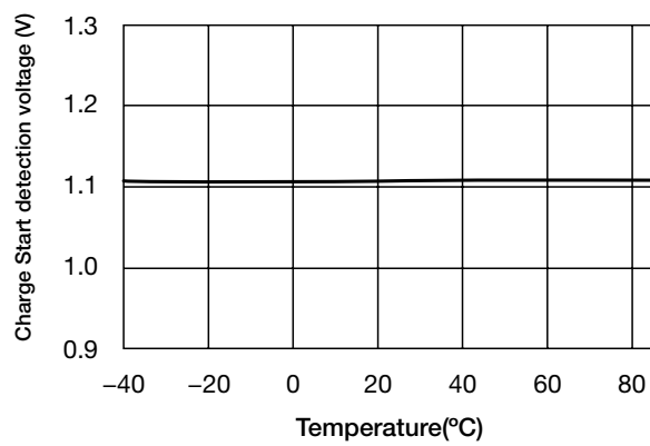
Charge Start detection voltage
